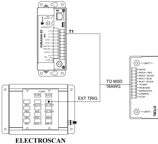
FIG 6 WIRING FOR SMART TOILET CONTROL WITH MSD
